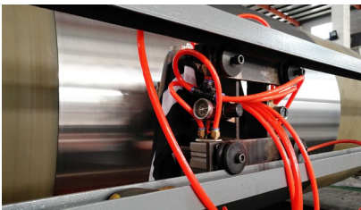
喷丸 Shot peening
